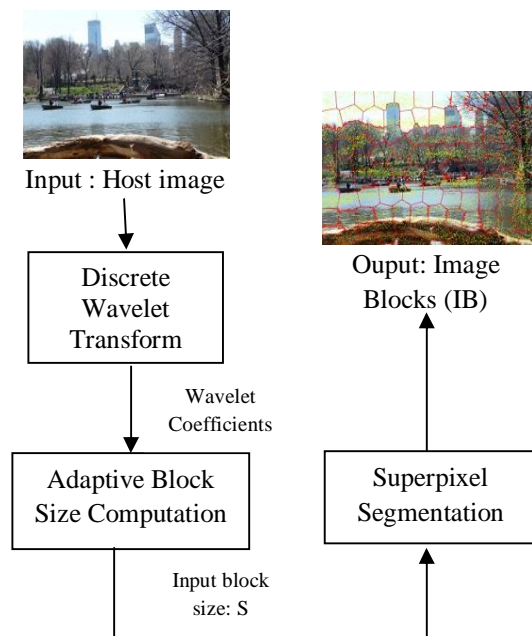
Fig.2: The adaptive over-segmentation flowchart
