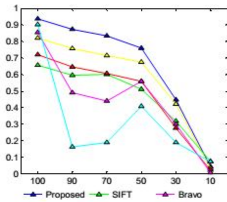
Fig. 5: Recall results at the pixel level (a) Down-sampling; (b) Scale; (c) Rotation; and (d) JPEG Compression
