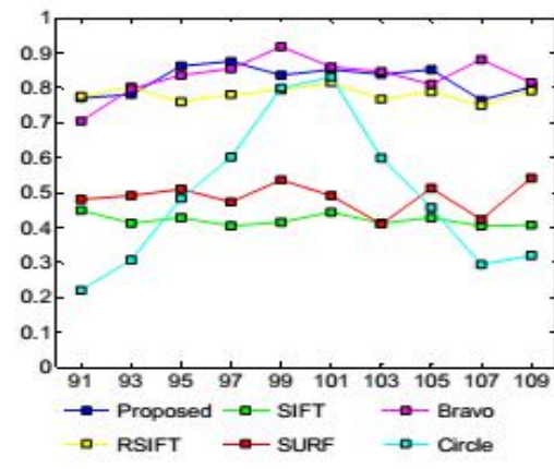
(b) Scaling
