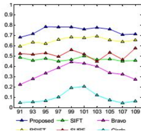
Fig. 5: Recall results at the pixel level (a) Down-sampling; (b) Scale; (c) Rotation; and (d) JPEG Compression
