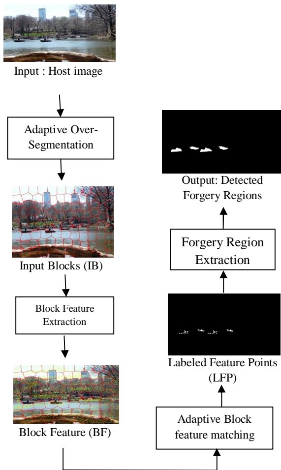
Fig.1: The proposed copy-move forgery detection scheme framework
