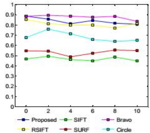
(c) Rotation
