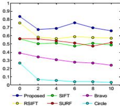
(c) Rotation
