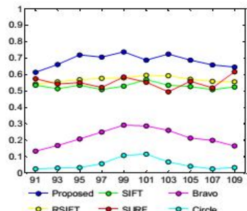
(b) Scaling
