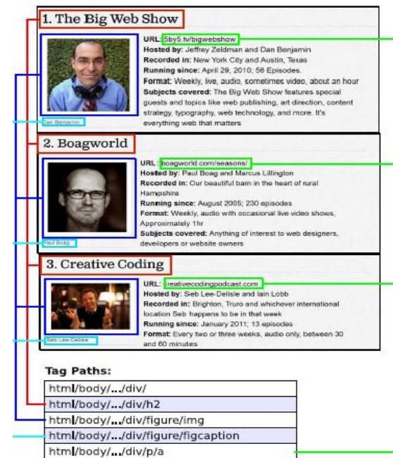
Fig.3 List nodes and their tag paths
