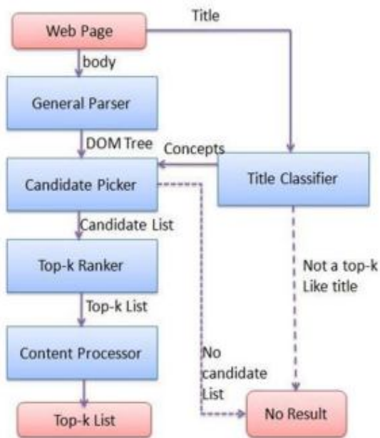
Fig. 2 System architecture
