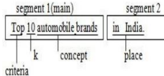
Fig. 1 Top-k title
