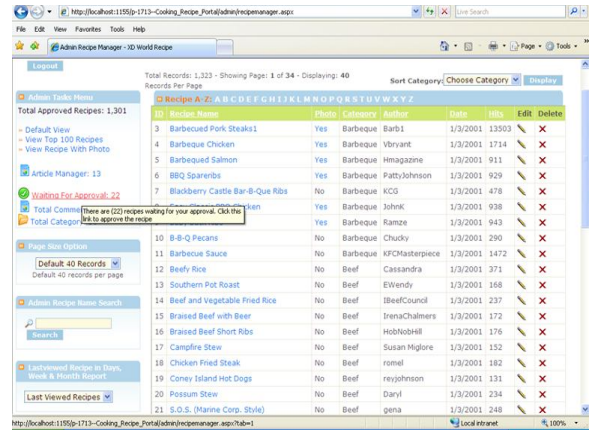
Fig.6 table pattern
