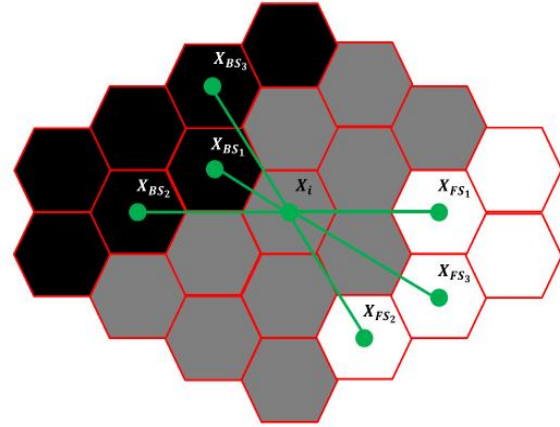
Fig.1. an illustration of local saliency features. Black, white, and gray regions denote background super pixels, foreground super pixels, and unknown super pixels, respectively. Use K -nearest foreground super pixels and K -nearest background super pixels to calculate a feature vector.
