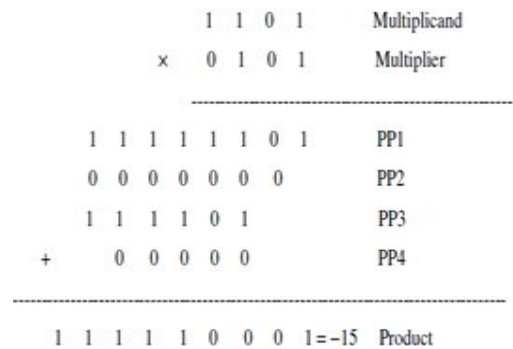
Fig 1.General multiplier
