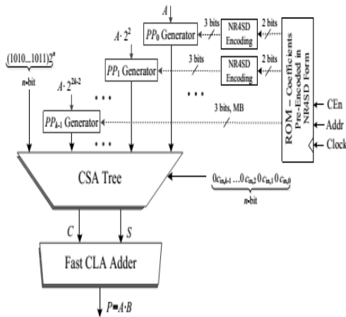
Fig.4 .System Architecture of the NR4SD Multipliers
