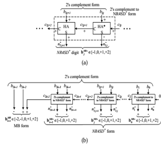
Fig.3. Block Diagram of the NR4SD + Encoding Scheme at the (a) Digit and (b) Word Level.
